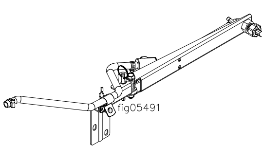
Right Broadcast Boom Assembly (Qty 1)
